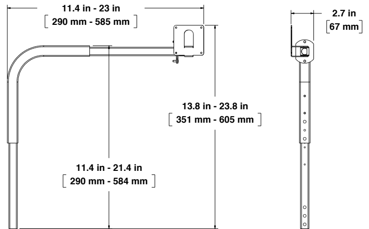
MM-PVM08GUX-W GONDOLA UPRIGHT MOUNT
