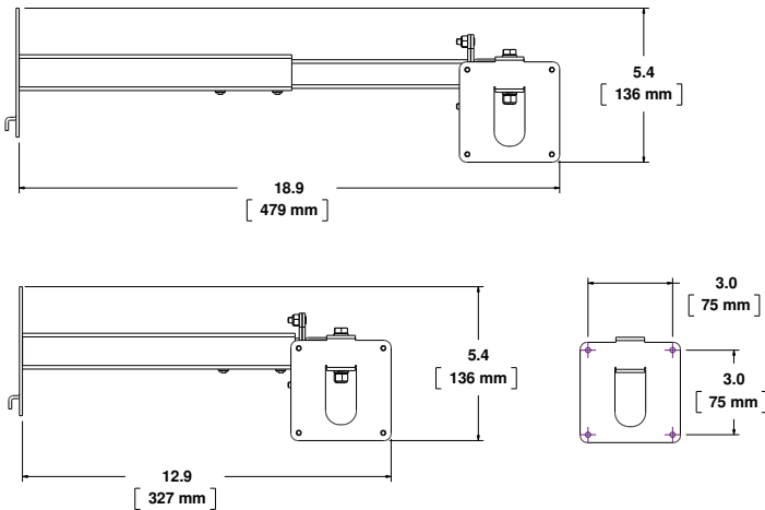
MM-PVM08CWA-W HORIZONTAL GONDOLA MOUNT
